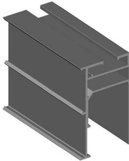
AZ0119- SECTIONAL DOOR SQUARE (AZ0071-2)
